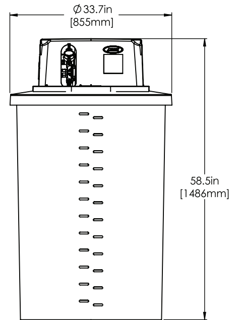
MIXING & STORAGE TANK
