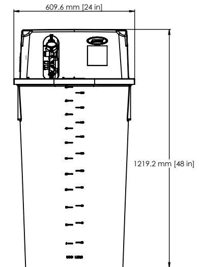
MIXING & STORAGE TANK 60 USG (227 LITRES)
