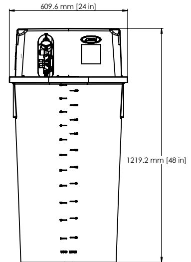
MIXING & STORAGE TANK 60 USG (227 LITRES)
